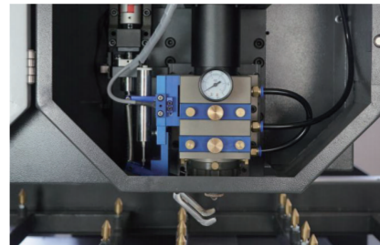
Laser head
